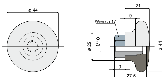
Round handle Part. 337 ( \varnothing 44 mm)
